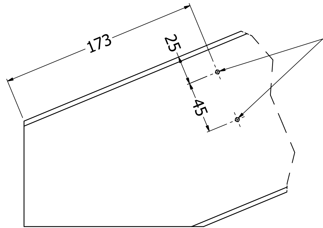
Detail E
